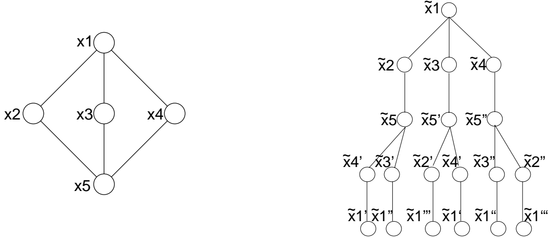
Fig. 3. a: A Markov Random Field with multiple loops. b: The unwrapped graph corresponding to this structure. The unwrapped graphs are constructed by replicating the potentials \Psi(x_i, x_j) and observations y_i while preserving the local connectivity of the loopy graph. They are constructed so that the messages received by node x_1 after t iterations in the loopy graph are equivalent to those that would be received by x_1 in the unwrapped graph. An observed node, y_i , not shown, is connected to each depicted node.
