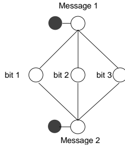
Fig. 4. Turbo code structure
