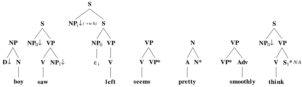
Figure 1: Example LCFG trees.
