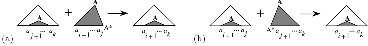
Figure 5: (a) Left concatenation and (b) right concatenation.
