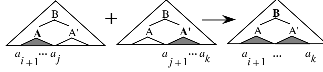
Figure 4: Sibling concatenation.
