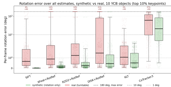
Figure 2: Rotation error over all per-frame estimates, aggregated over the 10 YCB objects, for the top 10% of keypoints. The green box is the synthetic sequence, built by rotating the reference frame, the pink box is the real turntable sequence. Each box shows the interquartile range, the whiskers reach the 5th and 95th percentiles, and the faint points are the individual estimates. The dashed lines mark 180^\circ and 10^\circ , the dotted line 1^\circ . The percentage above each method is the share of its real estimates past 90^\circ .
