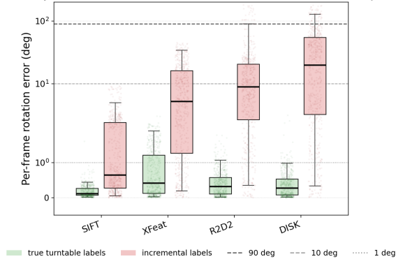
Memory-bank rotation error, true vs incremental labels, 10 YCB objects
