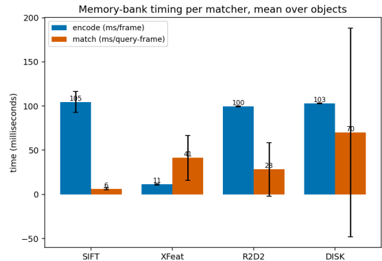
Figure 4: Per-frame timing of the MS, mean over the 10 YCB objects, at a working resolution of 1600 pixels. The blue bar is the time to encode one frame, the orange bar the time to match one query frame against the whole MS. End-to-end cost is the two added. SIFT is cheapest to match but slowest to encode, XFeat the reverse and fastest end to end. The wide spread on the DISK match bar comes from one textured object that detects far more keypoints than the rest, and the match cost grows with the square of the keypoint count.
