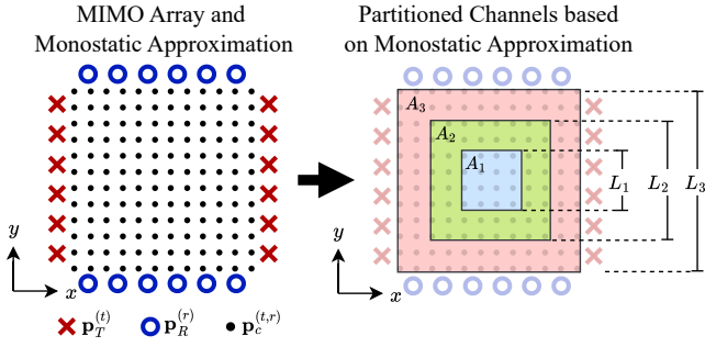
Fig. 1: Schematic diagram of partitioning MIMO channels based on cross-range resolution.
