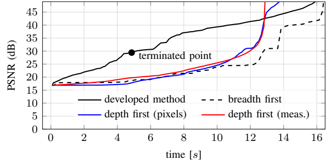
Fig. 3: PSNR with respect to runtime.
