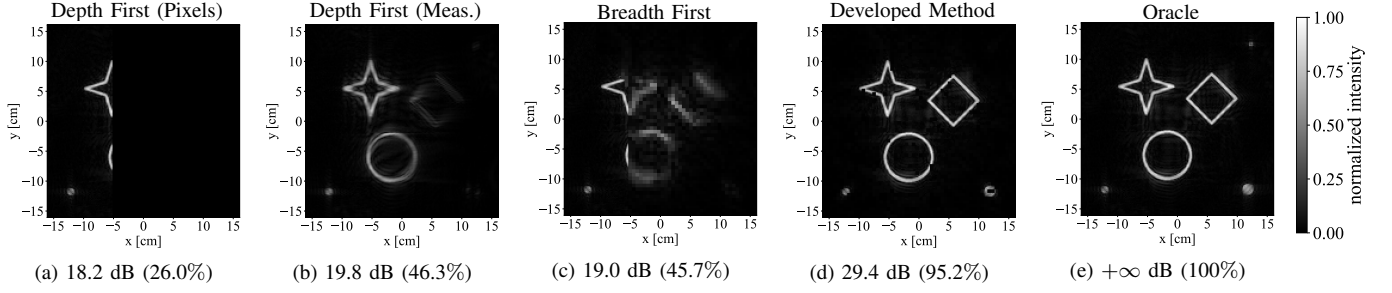
Fig. 5: The reconstructions at the termination point are shown in (a)-(d) while the oracle reconstruction is shown in (e). The PSNR and the recovered energy (in parentheses) are indicated below each reconstruction.
