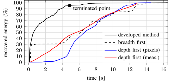
Fig. 4: Recovered energy with respect to runtime.
