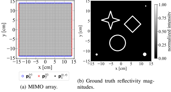
Fig. 2: Simulated MIMO array and the scene.
