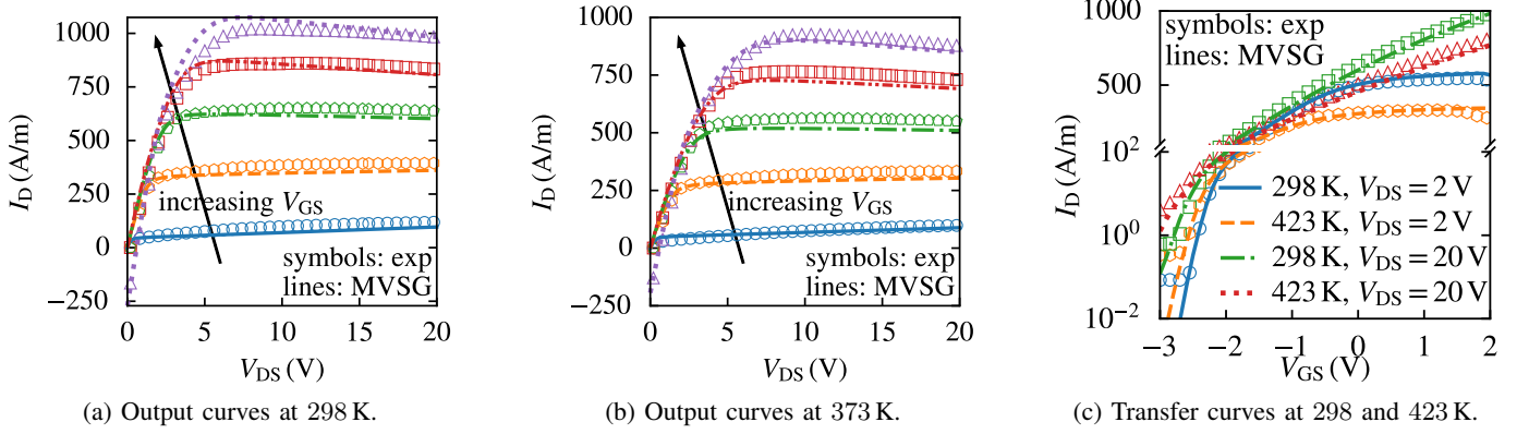
Fig. 2. Measured and simulated DC I-V characteristics at various baseplate temperatures. Output curves are for V_{GS} = \{-2, -1, 0, 1, 2\} V.
