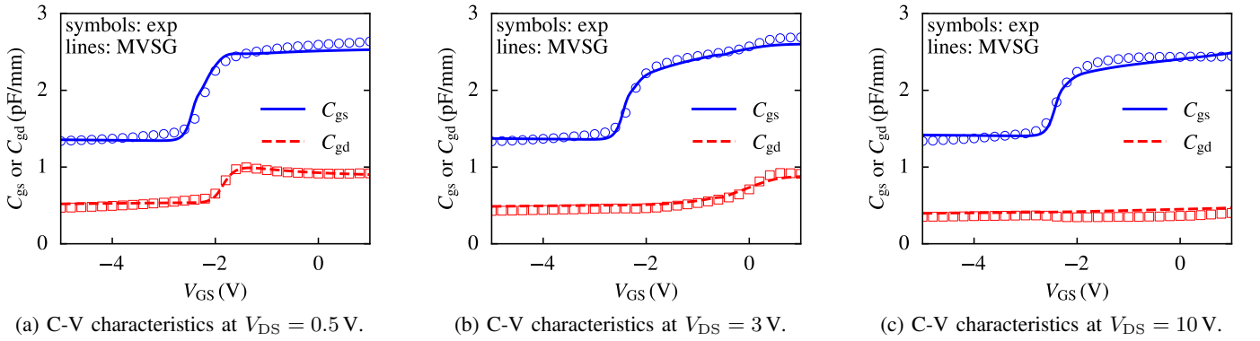
Fig. 3. Measured and simulated C-V characteristics calibrated at 298 K.
