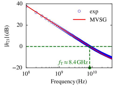
Fig. 6. Measured and simulated current gain vs. frequency calibrated at V_{DS} = 30 V and I_D = 0.015 A, i.e., V_{GS} = -2.5 V. f_T \approx 8.4 GHz.
