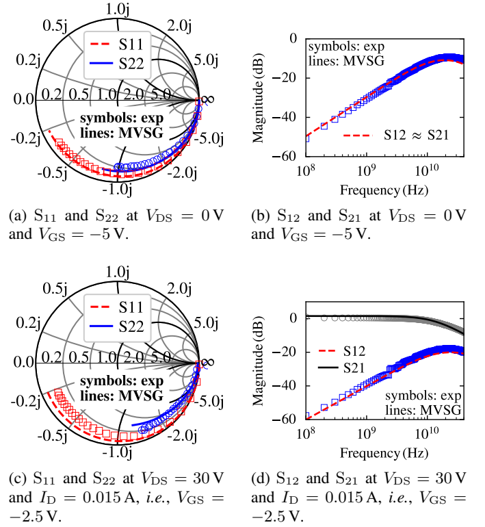
Fig. 5. Measured and simulated S-parameters from 0.1 GHz to 40 GHz calibrated at 298 K. See higher gate overdrive hot-device simulation results in Supplementary Material Sec. IV.
