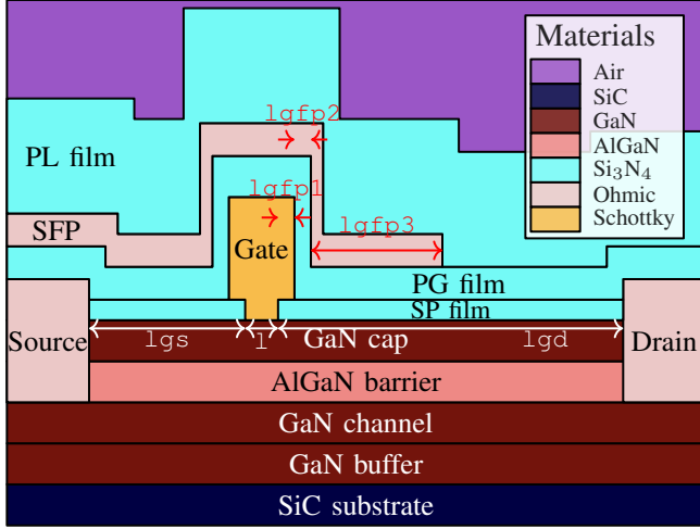
Fig. 1. Cross-section of the fabricated AlGaIn/GaN HEMT with labeled material layers. Drawing is not to scale. Only dimensions relevant to the MVSG-RF compact model are labeled. SFP: source field plate, SP: silicon nitride passivation, PG: gate passivation, PL: general passivation layer.
