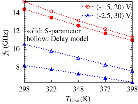
Fig. 9. Cutoff frequency vs. baseplate temperature formulated using both S-parameter directly from MVSG and using the simplified delay model. Symbols represent different (V_{\text{GS}}, V_{\text{DS}}) bias choices.
