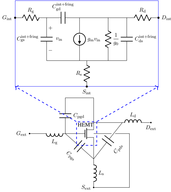
Fig. 4. Circuit schematics showing intrinsic device and lumped parasitic elements. Consult text and Table I for the meaning of various circuit elements.
