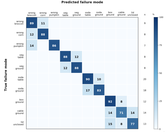
Fig. 7. VLM failure detector confusion matrix. Rows are normalized by the true failure mode, and the support column reports the number of physical-rollout occurrences used for each row.
