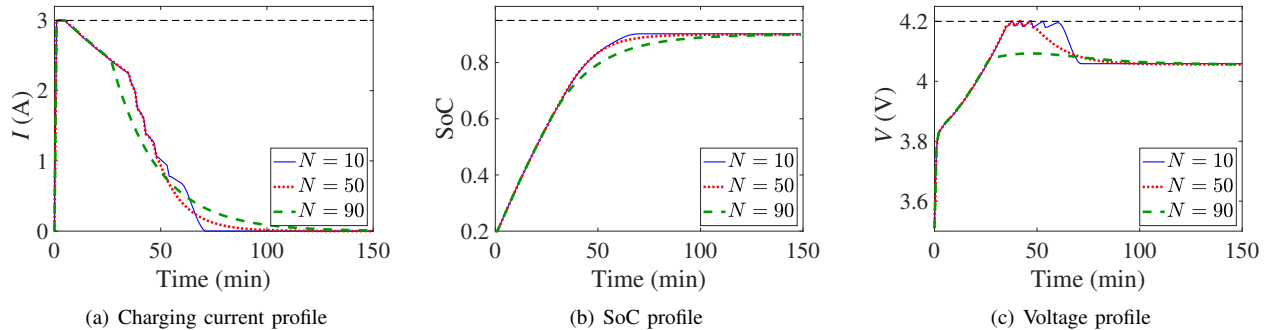
Figure 10: Charging control when the prediction horizon N = 10, 50, 90 .
