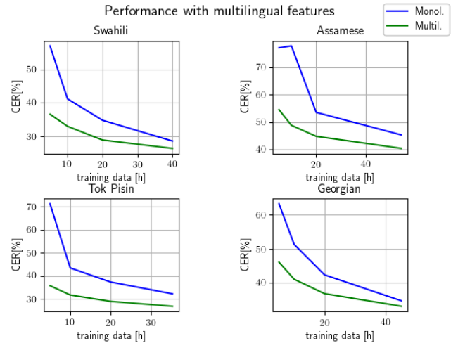
Figure 1: Performance of Monolingual models trained with multilingual features on different amount of data.
