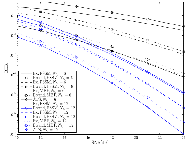
Fig. 2: BER performance for various transmission schemes with N_{ts} = 6 and N_{ts} = 12 .
