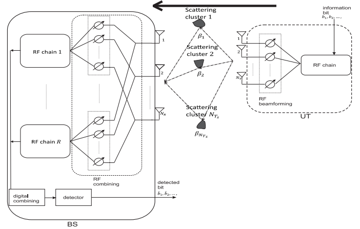
Fig. 1: Simplified architecture of the transmitter and receiver in uplink communications, where \beta_l denotes the gain of the l th scattering cluster.
