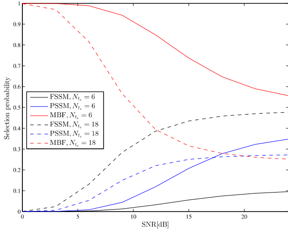
Fig. 4: Selection probability for non-adaptive transmission schemes.
