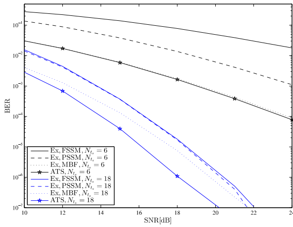
Fig. 3: BER performance for various transmission schemes with N_{ts} = 18 .
