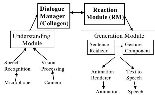
Figure 5.1: System architecture
