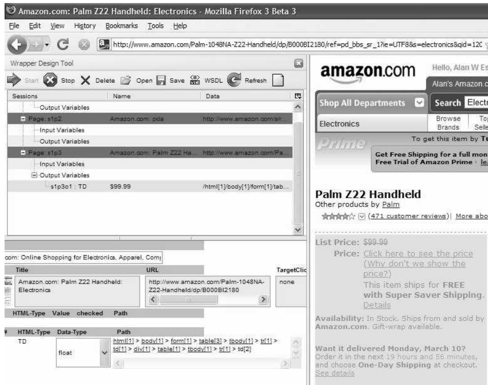
Figure 2: An interactive tool for construction of extraction rules for information extraction from web pages.
