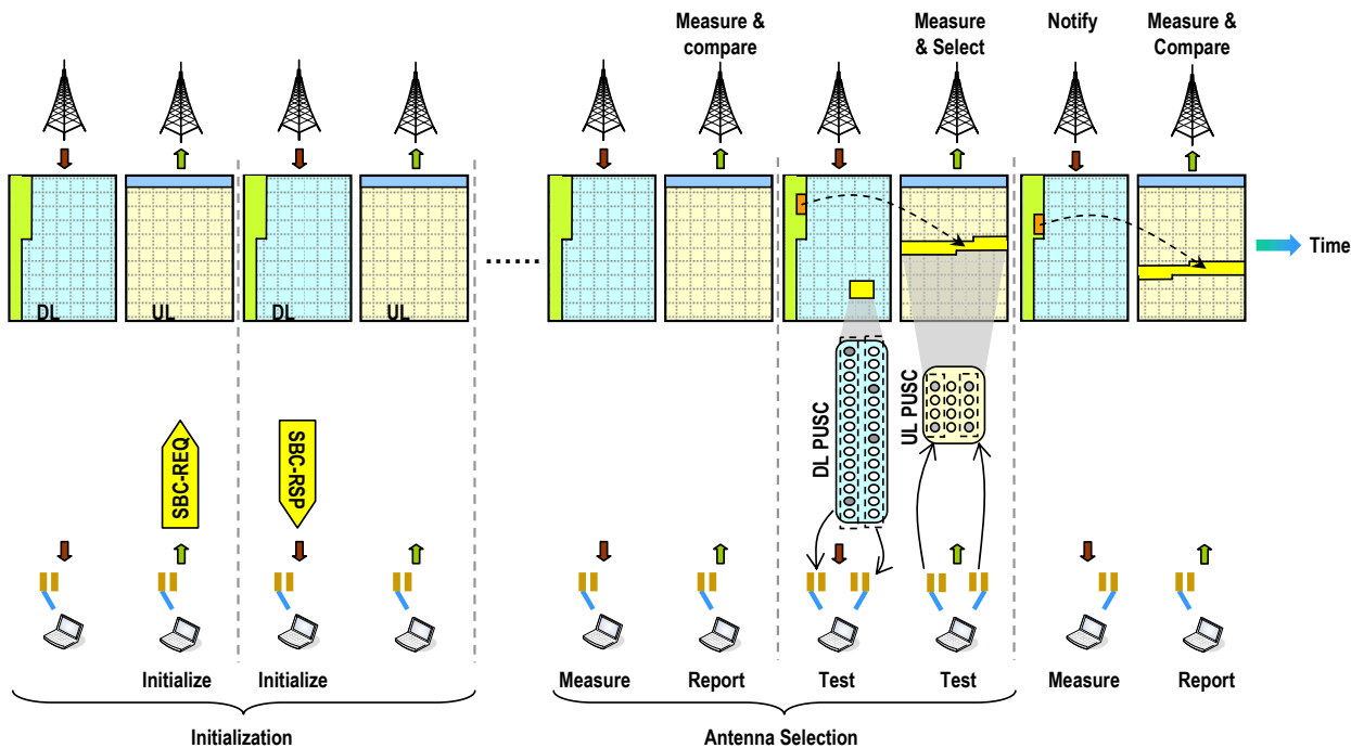
Fig. 3: Adaptive antenna selection protocol in the IEEE 802.16 system.
