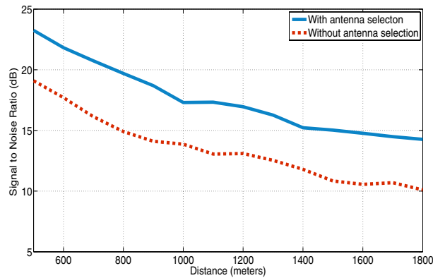
(a) Signal to noise ratio
