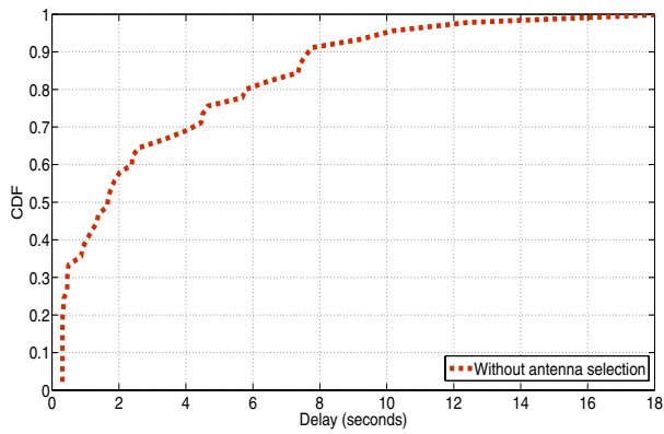
(a) Delay CDF without antenna selection
