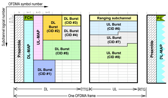
Fig. 1: OFDMA frame structure of the IEEE 802.16 TDD system.
