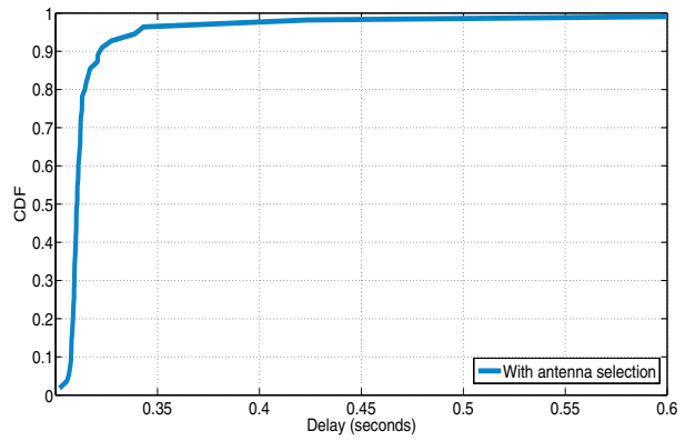
(b) Delay CDF with antenna selection
