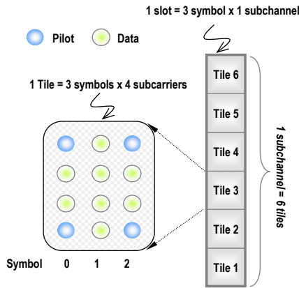
Fig. 2: PUSC permutation in IEEE 802.16.
