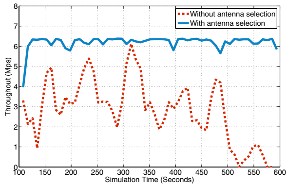
Fig. 4: Instantaneous throughput with ARQ.
