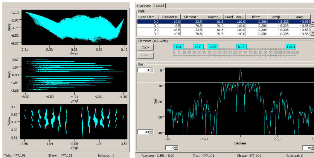
Figure 2: Visual browser with Overview Pane (left) and Inspect Pane (right).
