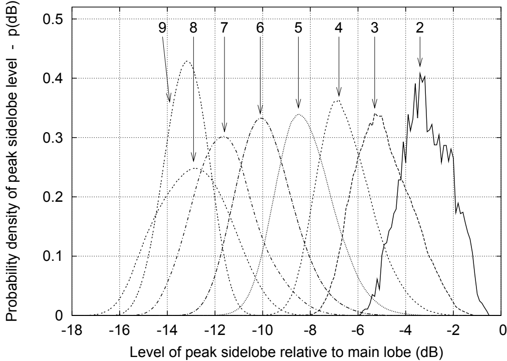
Figure 3: Histograms of the peak sidelobe level for configurations with 2 to 9 interior elements. The histograms have been normalized so that they integrate to 1, making them probability density functions.
