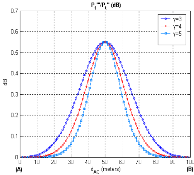
Fig. 2. Power savings of regenerating with respect to simple relaying at intermediate node positions over the direct path between A and B separated with 100m. Note: \Pr_e^{AB} = 10^{-3} , x_{AB}, x_{CB}, x_{AC} = 0 , M=64 , and (3P_c + 2P_{rec}(R)) / \alpha_R = 0.2 .
