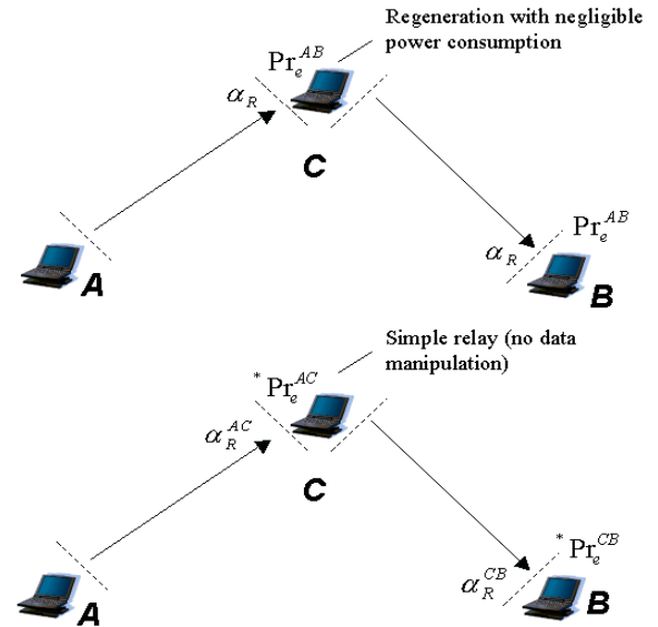
Fig. 1. Illustration of the received signal power levels and bit error rates at receiving terminals in wireless transmission over (top) the regenerator (bottom) simple relay intermediate node.
