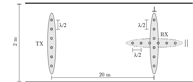
Fig. 1. Antenna measurement setup showing the receiver array setup parallel to the LOS ( \parallel ), and the receiver array setup perpendicular to the LOS ( \perp ).
