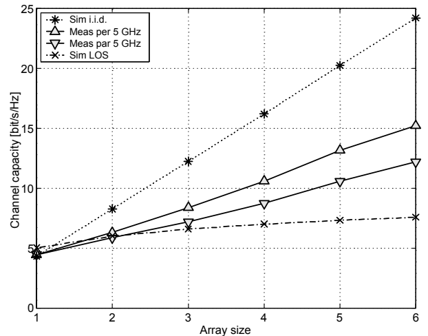
Fig. 2. Mean capacity for different array sizes ( N_R = N_T ) evaluated at a SNR of 15 dB.
