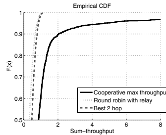
Fig. 5. CDF of sum throughput, max throughput criterion, random MS placement.
