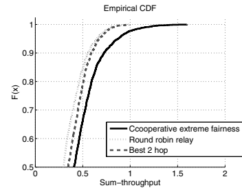
Fig. 6. CDF of sum throughput, the extreme fairness criterion, random MS placement.
