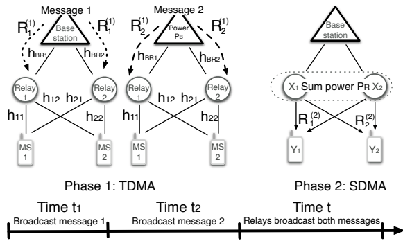
Fig. 1. Transmission takes place in two phases: in phase 1 the BS broadcasts messages in TDMA fashion: message W_1 for t_1 time units, then message W_2 for t_2 time units. During phase 2 the relays simultaneously transmit all received messages to the mobiles. Illustrated are the channel gains, power constraints, rates, and input-output variables.
