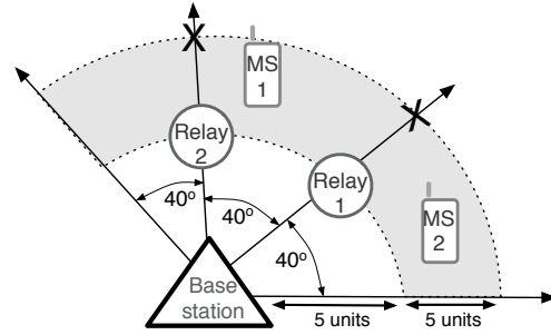
Fig. 3. Geometric distribution: relays at equal distance, spaced at angles 40^\circ on arc of radius 5 units, mobiles random in shaded sector for the random MS placement, or at the points marked X for the fixed MS placement.
