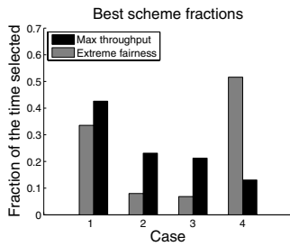
Fig. 4. Percentage of time the 4 cases are chosen, random MS placement. P_R = P_B = 1000 , radius=10 units.
