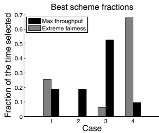
Fig. 7. Percentage of time the 4 cases are chosen, fixed MS placement. P_R = P_B = 1000 , radius=10 units.
