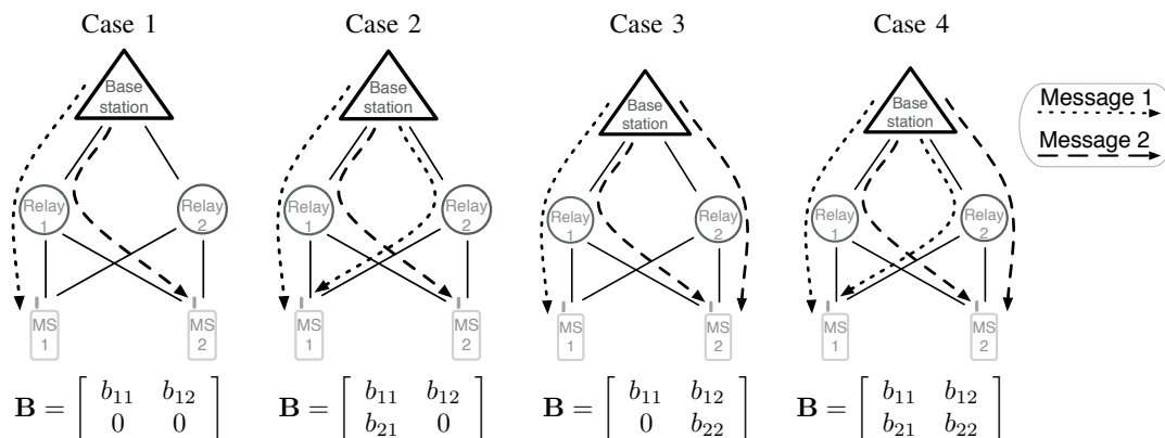
Fig. 2. Four message knowledge scenarios when |h_{BR_1}| \geq |h_{BR_2}| , and the corresponding linear precoding matrices \mathbf{B} .
