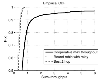
Fig. 8. CDF of sum throughput, max throughput criterion, fixed MS placement.
