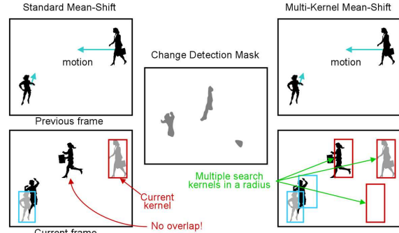
Fig. 2. We iterate the mean-shift in multiple kernels.
