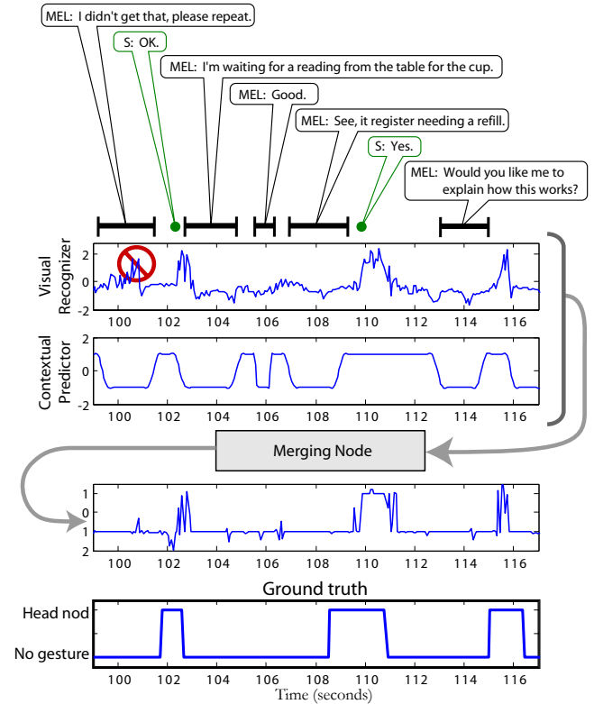
Figure 8: Head nod recognition results for a sample dialogue. The last graph displays the ground truth. We can observe at around 101 seconds (circled and crossed in the top graph) that the contextual information attenuates the effect of the false positive detection from the visual recognizer.
