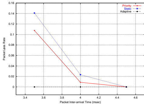
Fig. 3. Packet-loss rate
